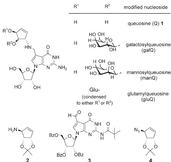
Scheme 1. Chemical structures of queuosine ( 1 ), its derivatives, and key synthetic intermediates. Bz = benzoyl.
