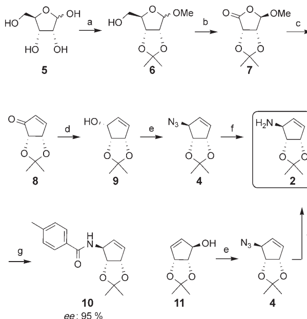
Scheme 2. Synthesis of the cyclopentenylamine 2 : a) 2,2-dimethoxypropane, MeOH, HClO 4 , acetone, 94%; b) PCC (4.0 equiv), benzene, reflux, 46%; c) (MeO) 2 P(O)CH 3 , n BuLi, THF, 0°C, 56%; d) NaBH 4 , CeCl 3 , MeOH, 0°C, 95%; e) DIAD, PPh 3 , HN 3 (1.3 M in toluene), THF, 0°C; f) PPh 3 , THF, 0°C, 72% (65% from 11 ) in two steps; g) toluoyl chloride, NEt 3 , CH 2 Cl 2 , 60%. PCC = pyridinium chlorochromate, DIA-D = diisopropylazodicarboxylate.
