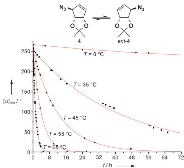
Figure 1. [3,3] sigmatropic rearrangement of 4 at T=0, 35, 45, 55 , and 65^\circ\text{C} in EtOH.
