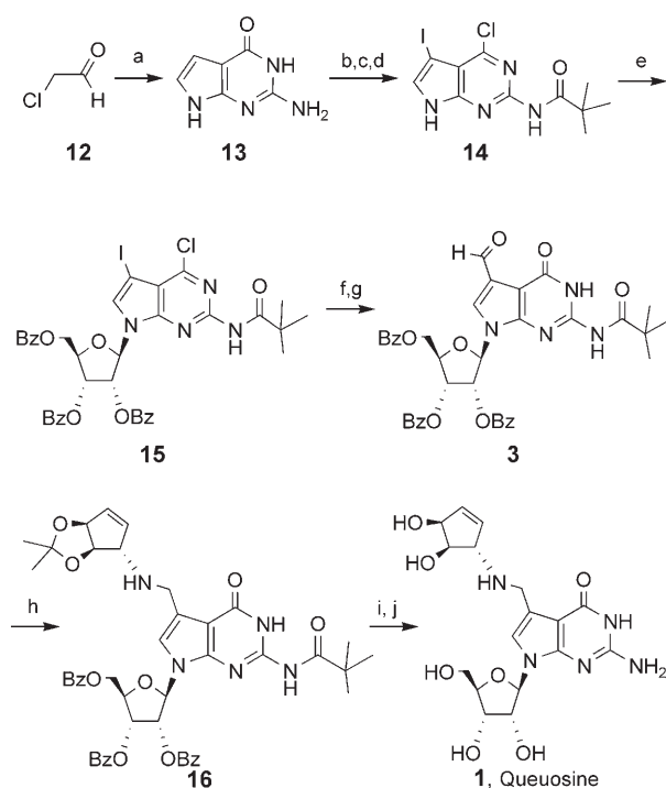
Scheme 3. Synthesis of queuosine ( 1 ): a) 1) NaOMe, H 2 O, DMF; 2) 2,4-diamino-6-hydroxypyrimidine, NaOAc, 86%; b) POCl 3 , 120 °C, 78%; c) PivCl, pyridine, 64%; d) NIS, THF, 81%; e) BSA, TMSTf, 1-O-acetyl-2,3,5-tri-O-benzoyl-D-ribofuranose, MeCN, 60%; f) DABCO, NEt 3 , CsOAc, DMF, 63%; g) [Pd 2 (dba) 3 ] PPh 3 , CO, Bu 3 SnH, 73%; h) 2 , benzene, then NaBH 4 , EtOH, 85%; i) NaOH, MeOH; j) HCl (2 N), 45%. Piv = pivaloyl, NIS = N -iodosuccinimide, BSA = bis(trimethylsilyl)-acetamide, TMSTf = trimethylsilyltriflate, DABCO = 1,4-diazabicyclo-[2.2.2]octane.
